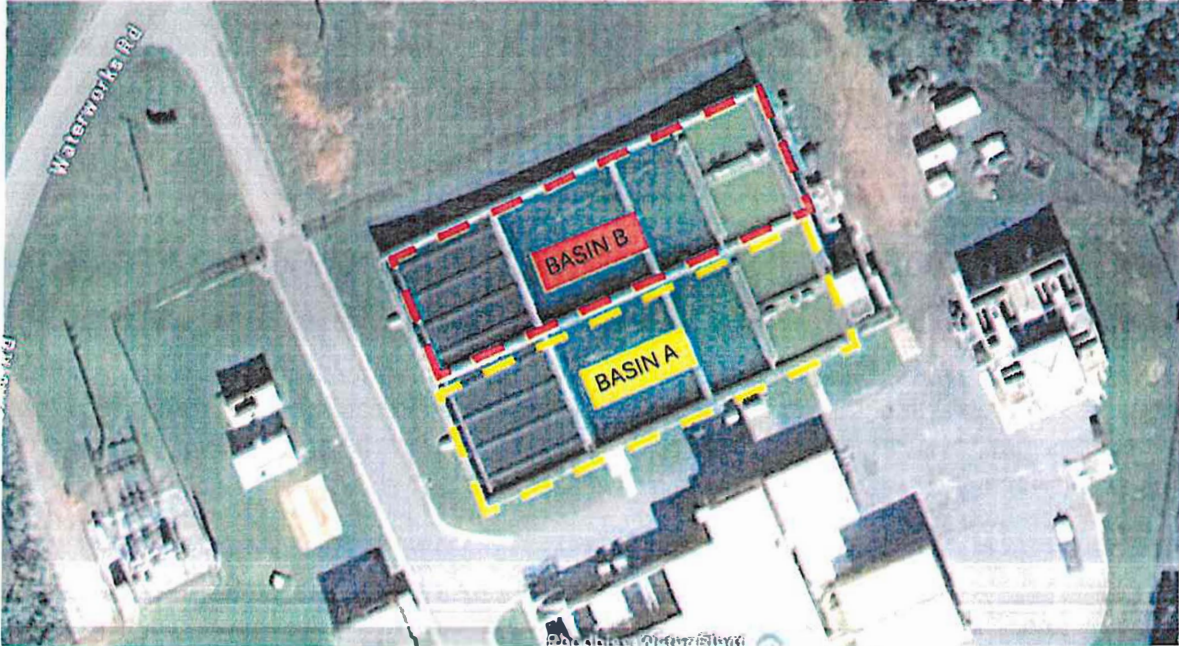
Figure 1. Plan view of the Lenoir WTP Exterior Basins. The Basins are split into 2 sides capable of independent operation. The south side, referenced as Basin "A", is outlined in yellow. The north side, referenced as Basin "B", is outlined in red. Basin "A" was evaluated in 2018 along with the Flash Mixer tanks currently under repair.
