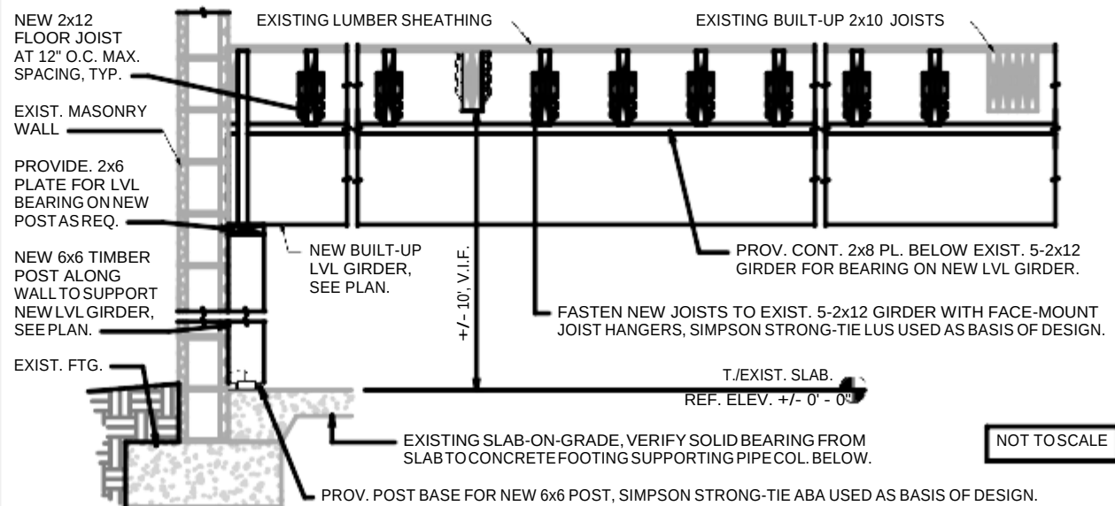
4 CONCESSIONS FLOOR REINFORCEMENT N/S SECTION AT WALL
